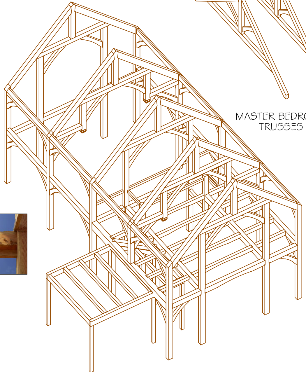
FRONT VIEW OF TIMBER SYSTEM- GREAT ROOM & DINING
