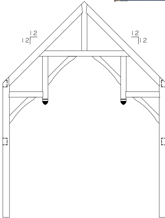
HAMMER BEAM BENT
